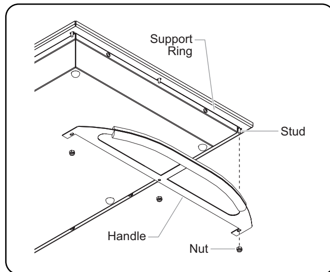
Handle Installation
