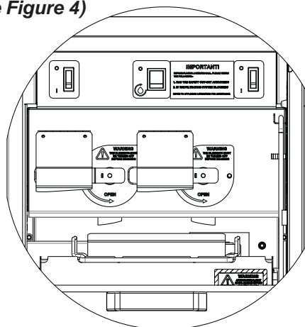
Figure 4 – All Models - Additional Controls
